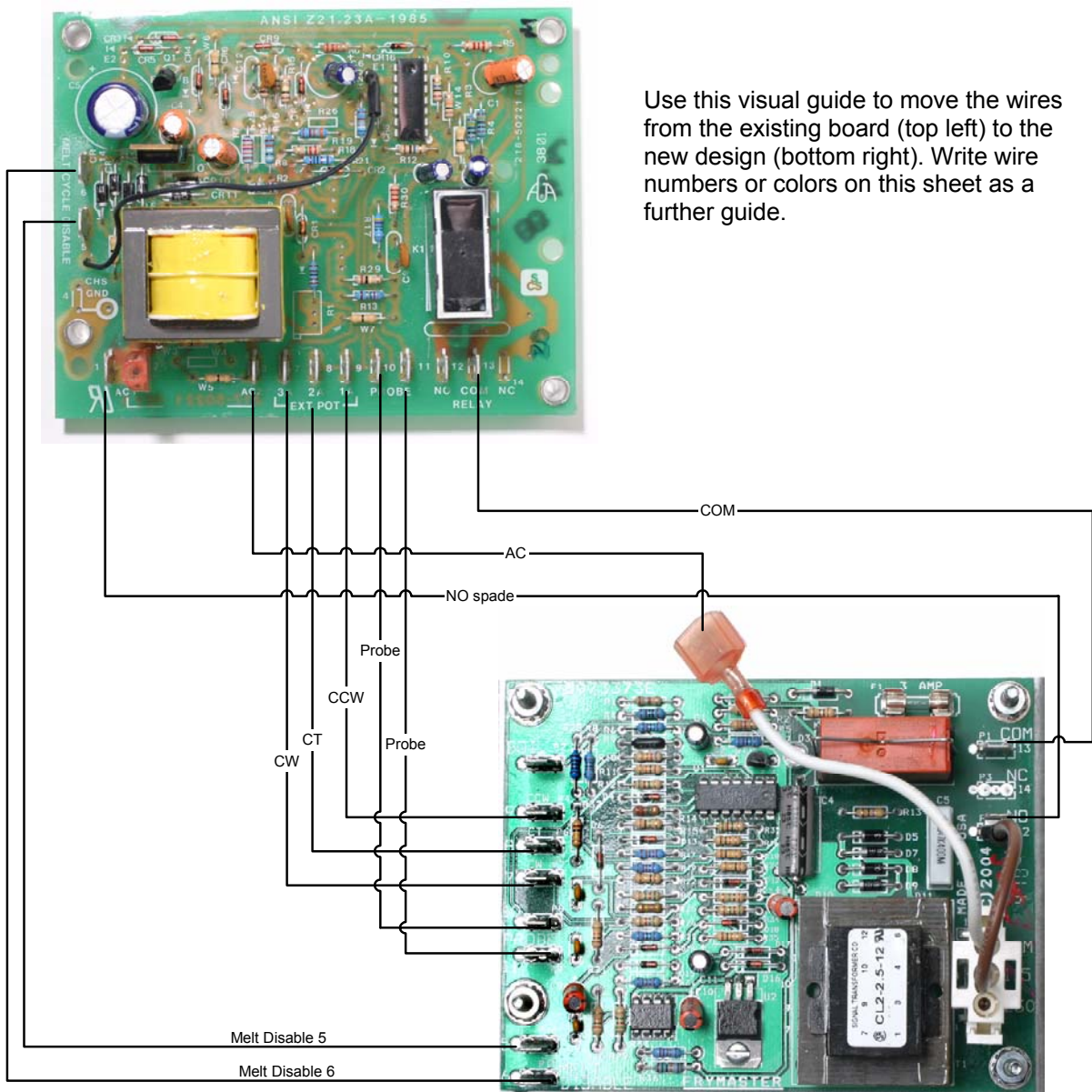
Figure 4: Route wiring to the new board as shown above.
